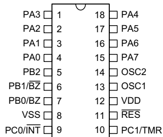
HT48R06A-1 - 18 DIP/SOP
